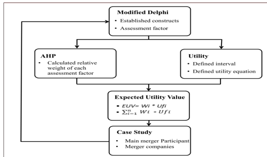
Figure 1. Flow of the application of the four decision theories.
