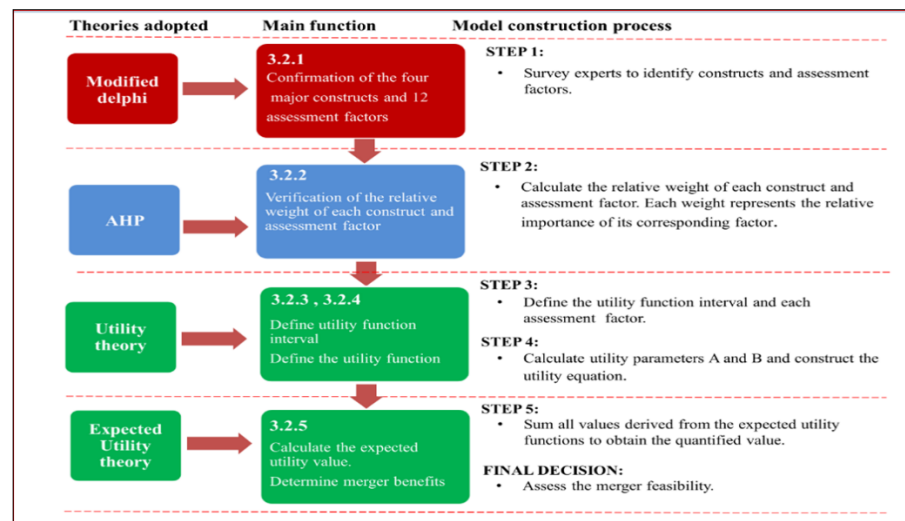
Figure 2. Flow of the six major steps.
